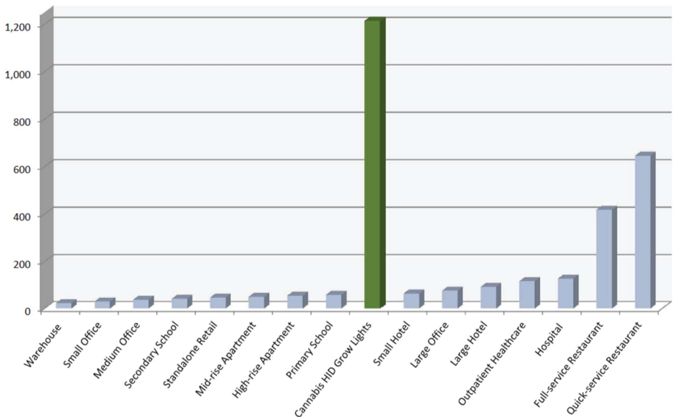
Figure 1. Energy Use Intensity (kBtu) per Square Foot. This graph identifies the energy use per square foot for cannabis production using HID grow lights as compared to other commercial and industrial uses. (Massachusetts Department of Energy Resources Energy and Environmental Affairs, 2018.)
