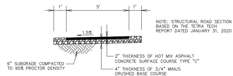
TEMPORARY ASPHALT SIDEWALK SECTION NO SCALE
