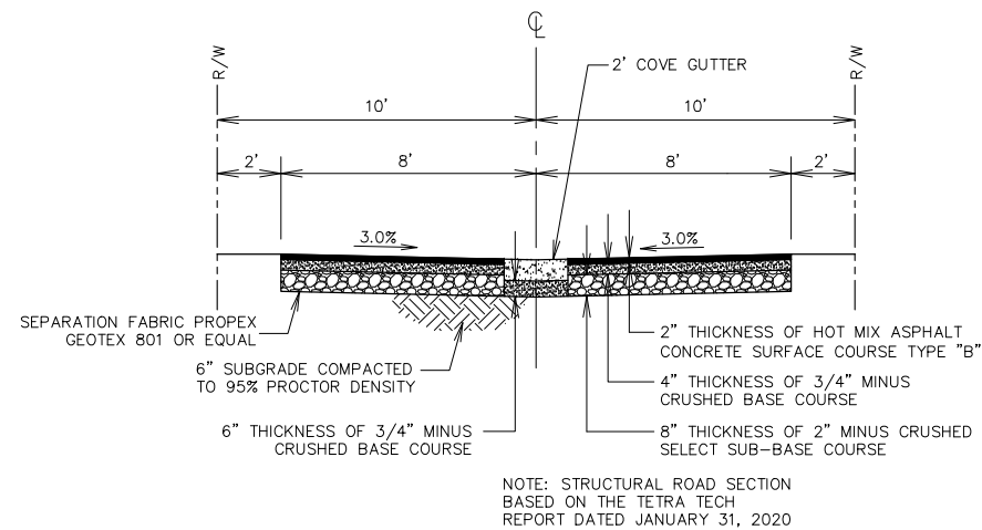
TYPICAL 16' ALLEY SECTION
