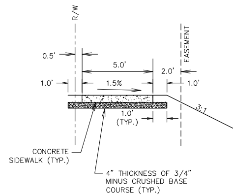
SIDEWALK A TYPICAL SECTION NO SCALE
