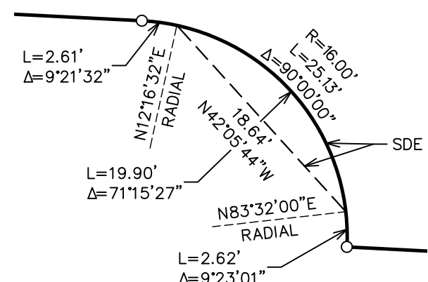
EASEMENT DETAIL NO. 2
