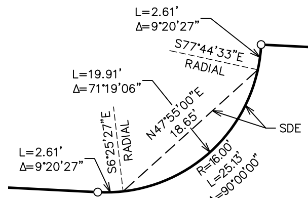
EASEMENT DETAIL NO. 1
