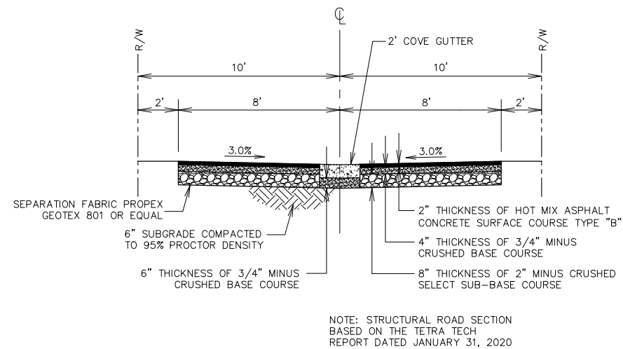
TYPICAL 16' ALLEY SECTION NO SCALE
