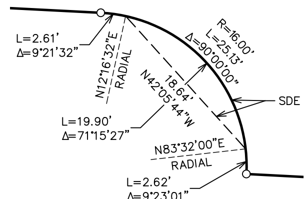
EASEMENT DETAIL NO. 2
