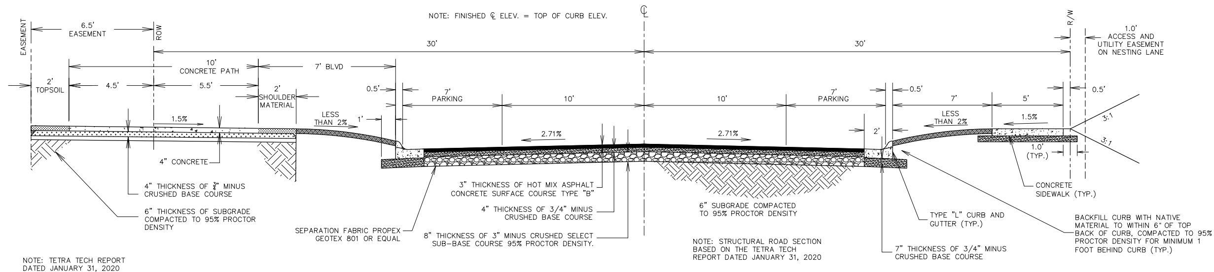
HERON'S LANDING DRIVE AND NESTING LANE STA. 9+66.25 TO 10+76.62 TYPICAL SECTION - LOCAL RESIDENTIAL STREET WITH 10' PATH NO SCALE
